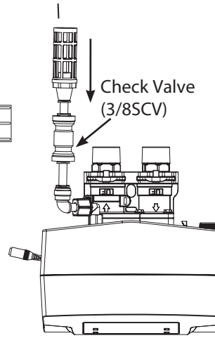
Screen Part # 60010244
